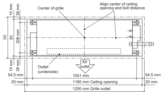
(a) 414 mm Grille out let (b) 384 mm Ceiling opening
